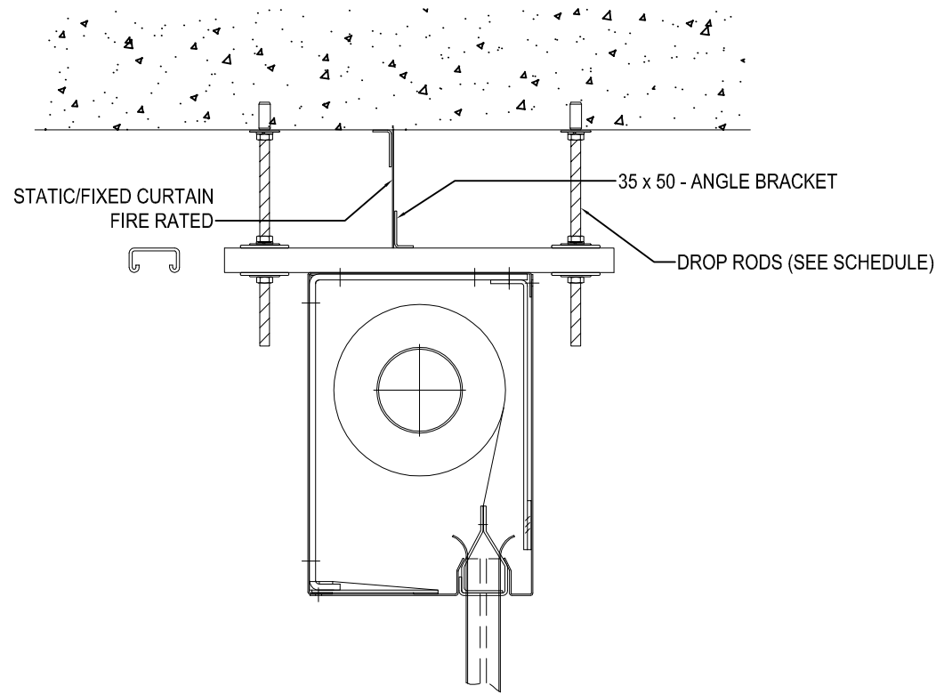
'DROP ROD' INTO SLAB FIXING
